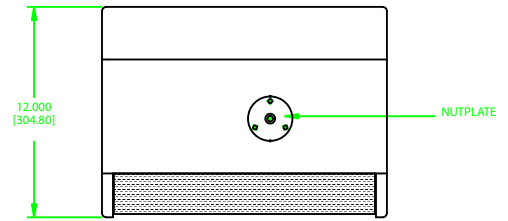
FRONT VIEW W/GRILL REMOVED
