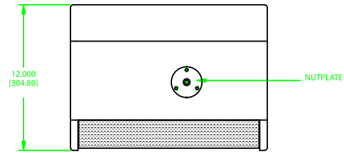
FRONT VIEW W/GRILL REMOVED
