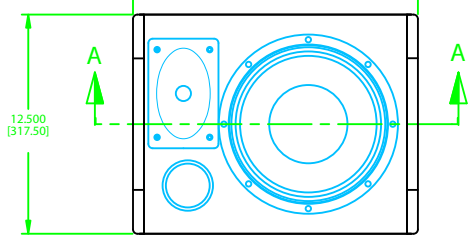
FRONT VIEW W/GRILL REMOVED
