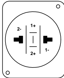
Neutrik NL4MP
