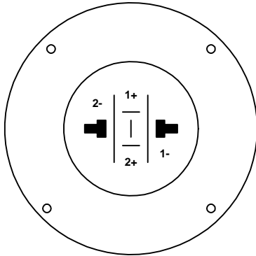
Neutrik NL4MPR
