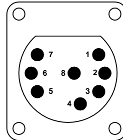
Cannon EP8 Series
