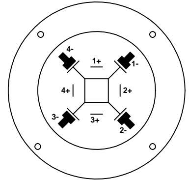
Neutrik NL8MP
